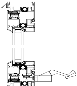
G1 Casement
