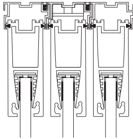
Clear Wall Slider Gasket TRANSLUCENT SILICONE
