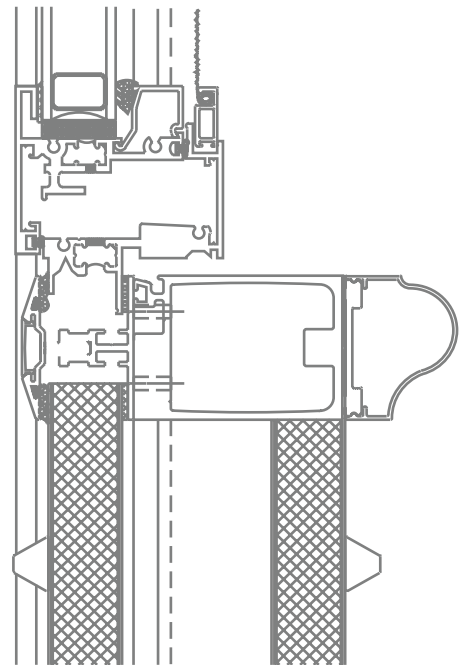
Insulated Panel Base wall with Exterior and Interior Grid
